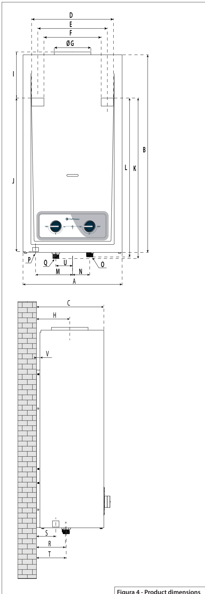
Figura 4 - Product dimensions
