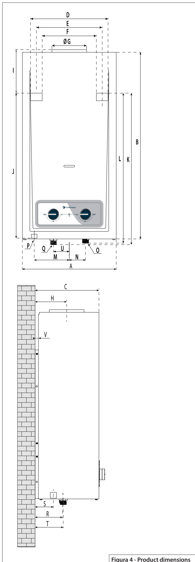
Figura 4 - Product dimensions
